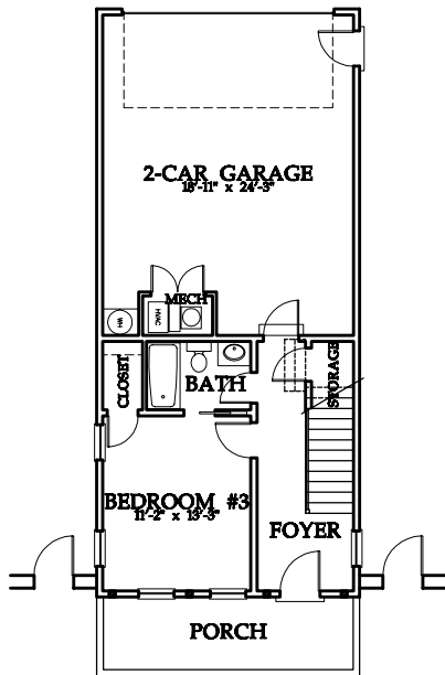
TERRACE LEVEL PLAN 8'-0" CEILING
